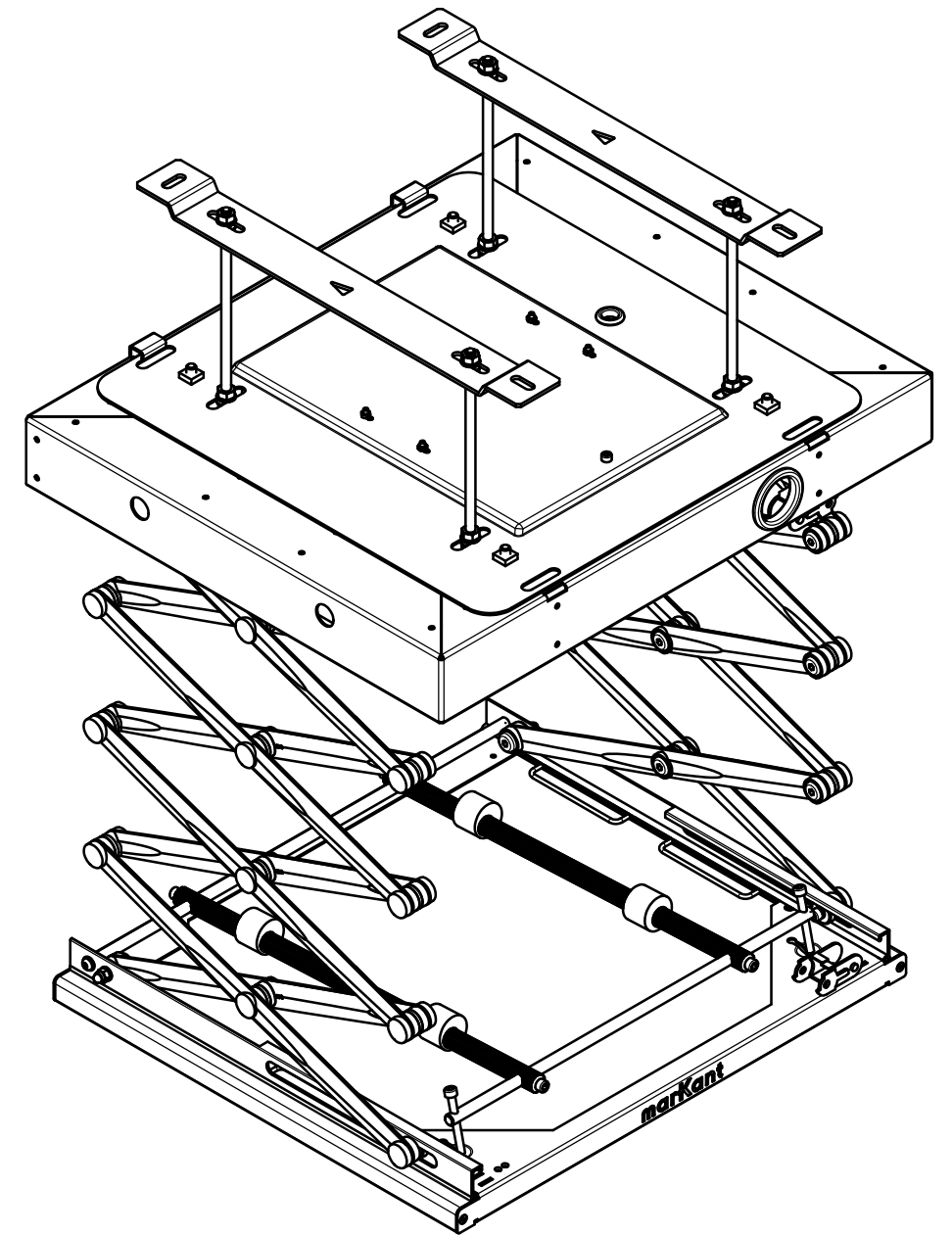
C-Lift XL
